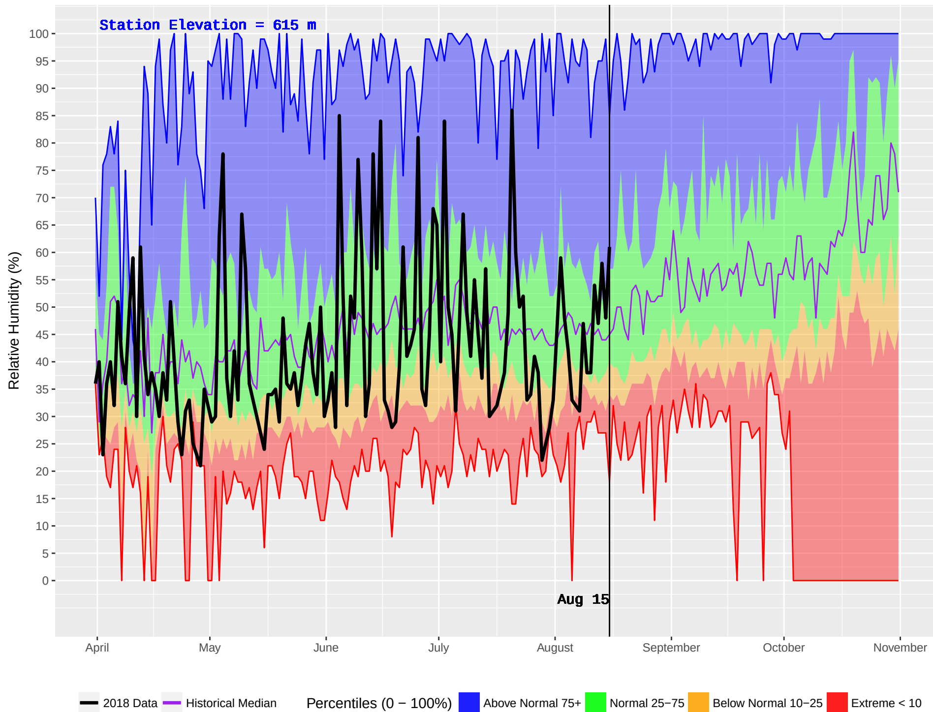
HIXON (187) : Historical (1976–2016) and Current (2018) Daily Relative Humidity
